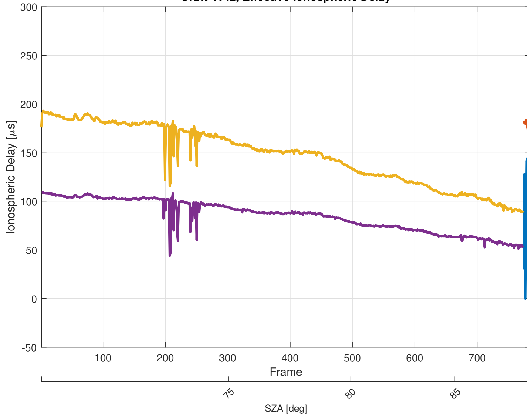
Orbit 4142, Effective Ionospheric Delay
