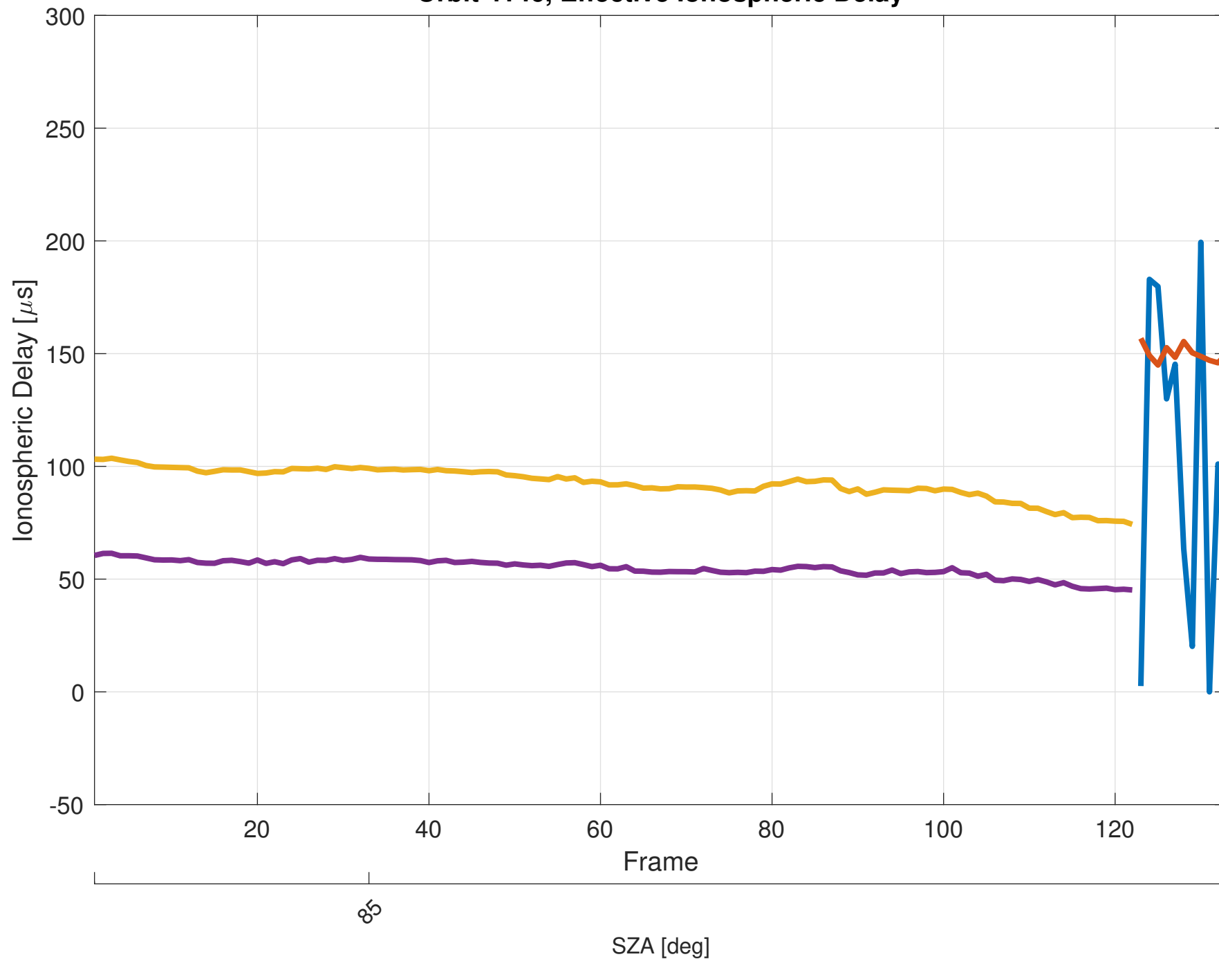
Orbit 4146, Effective Ionospheric Delay
