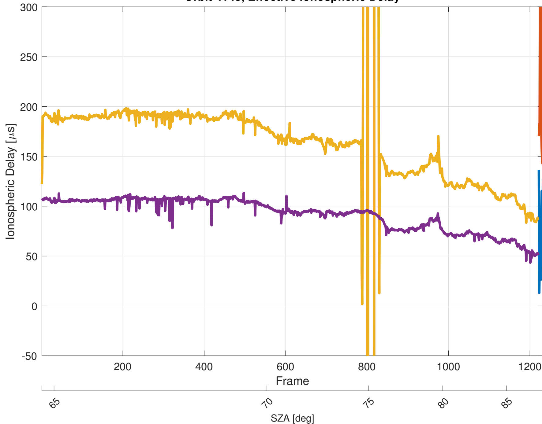
Orbit 4148, Effective Ionospheric Delay
