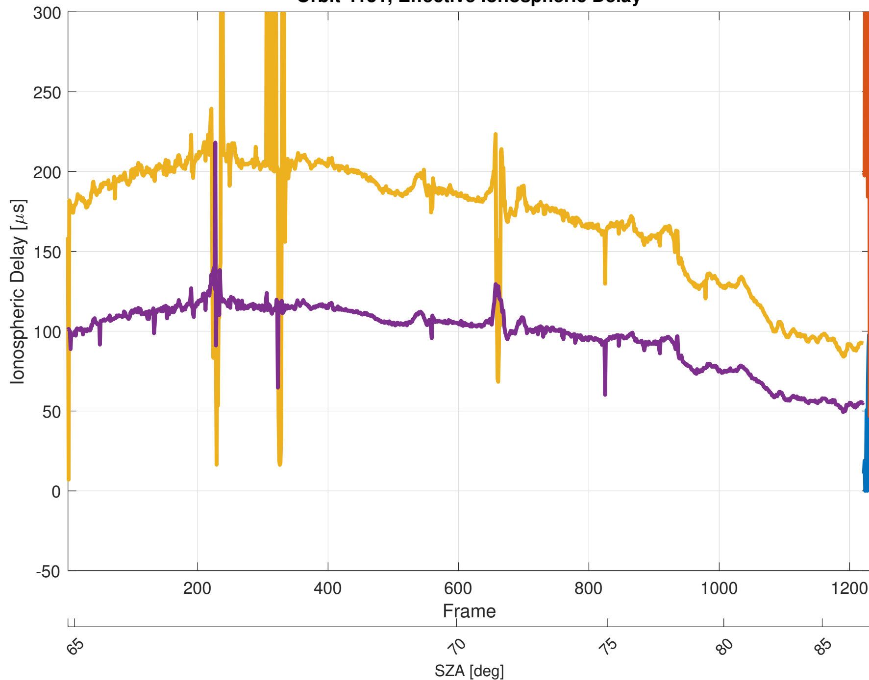
Orbit 4151, Effective Ionospheric Delay
