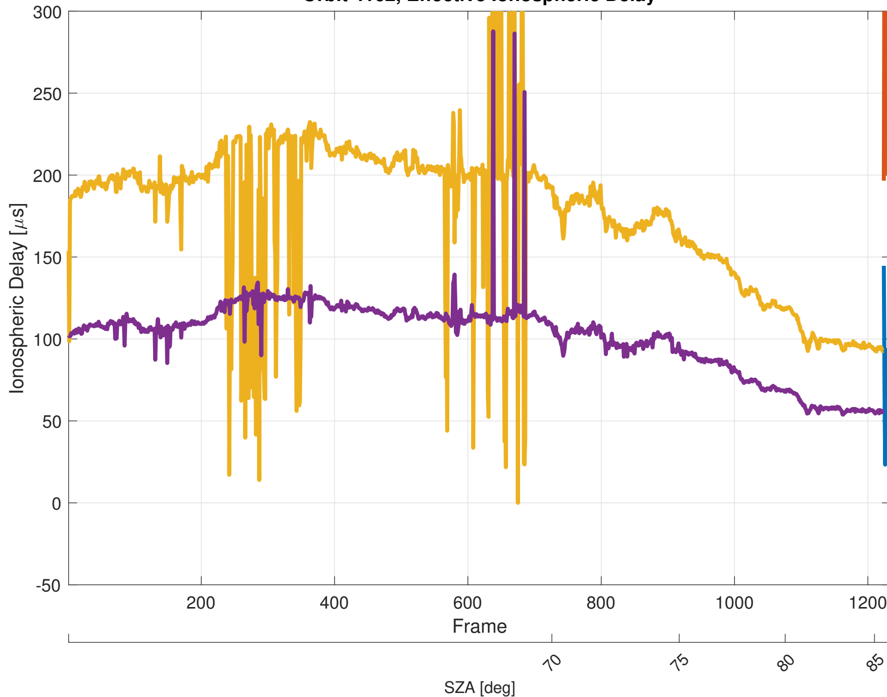
Orbit 4162, Effective Ionospheric Delay
