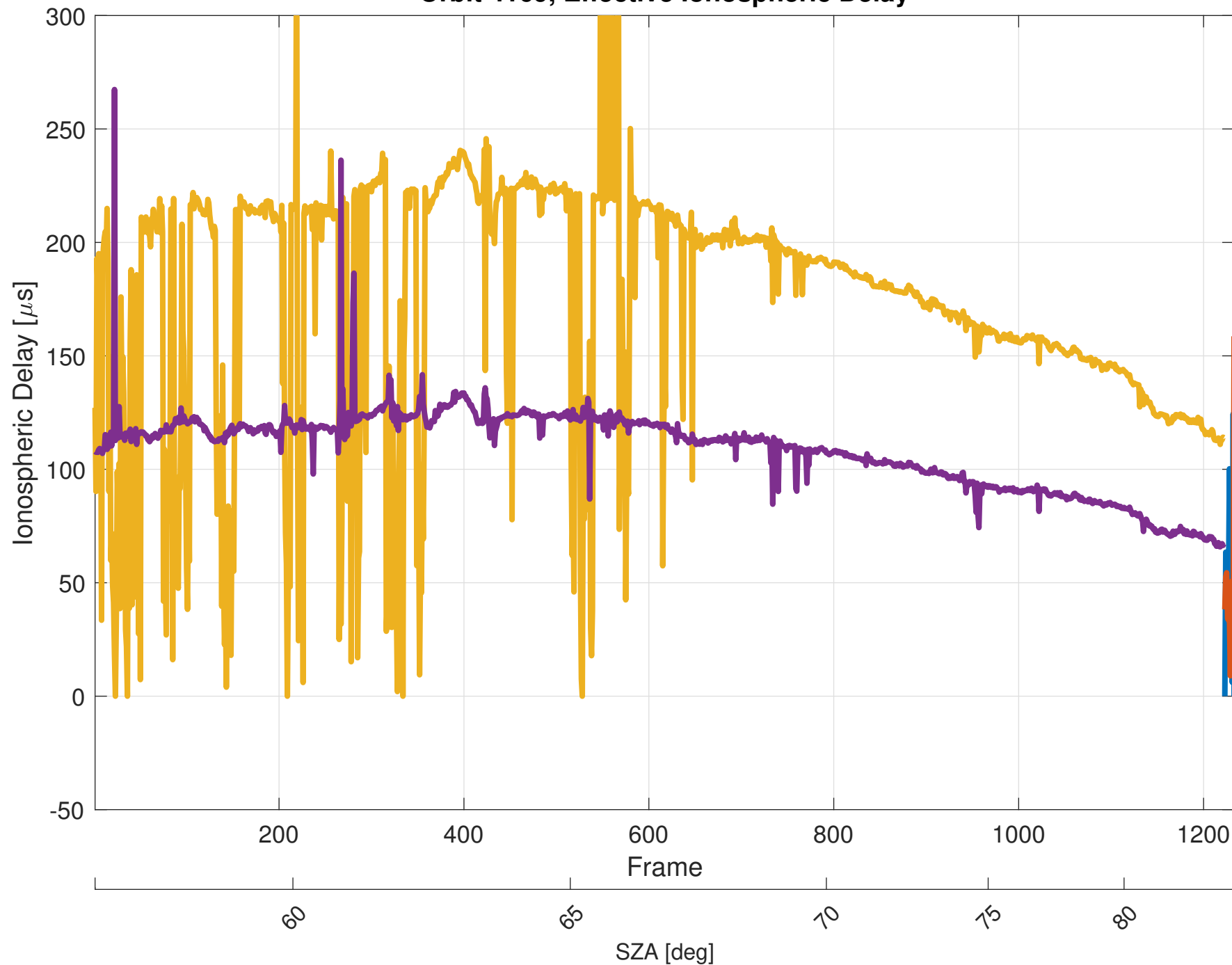
Orbit 4169, Effective Ionospheric Delay
