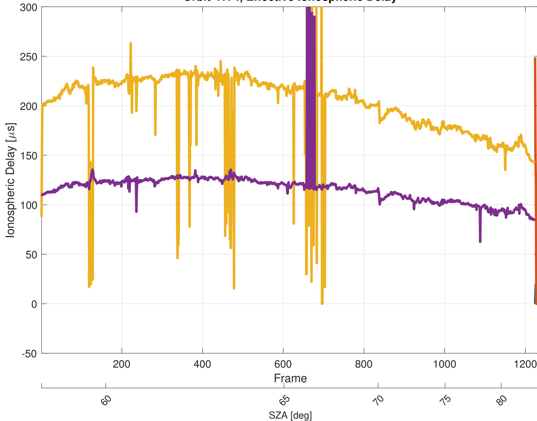
Orbit 4174, Effective Ionospheric Delay
