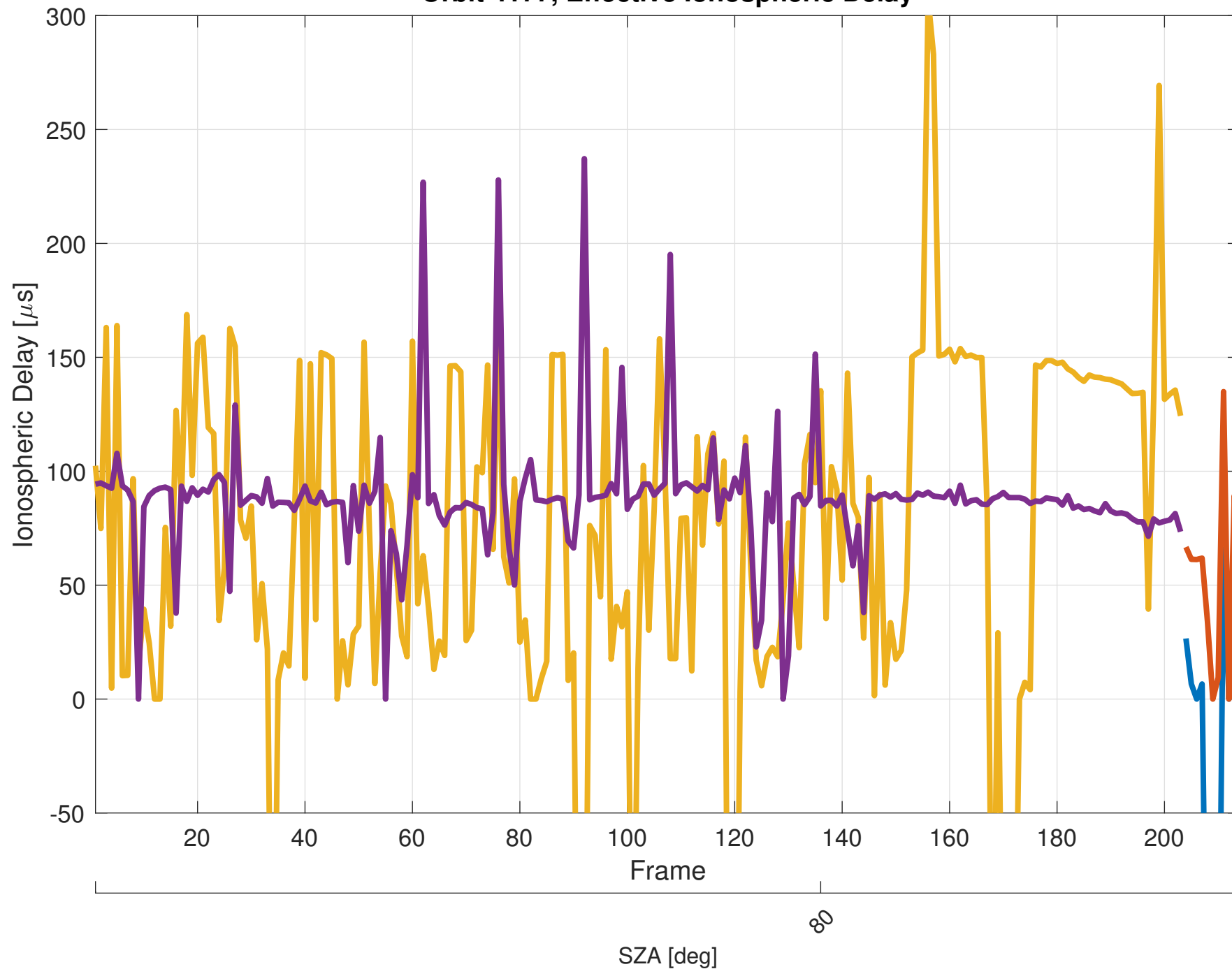
Orbit 4177, Effective Ionospheric Delay
