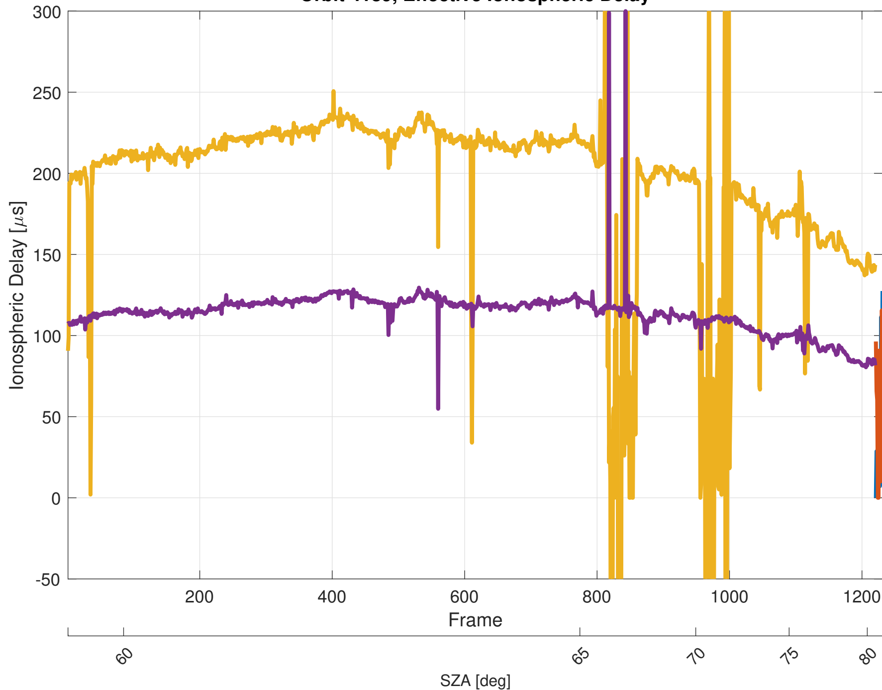
Orbit 4189, Effective Ionospheric Delay
