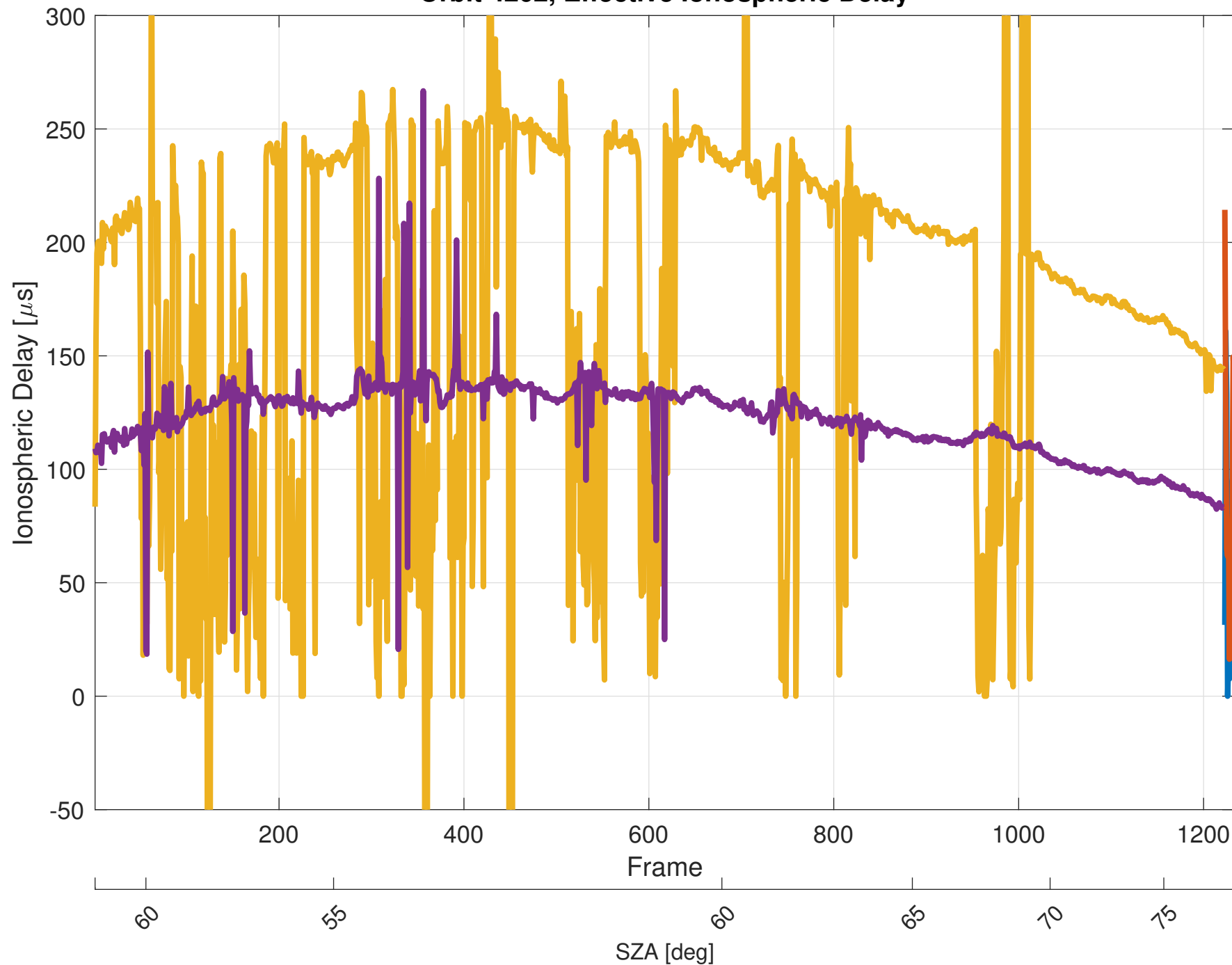
Orbit 4202, Effective Ionospheric Delay
