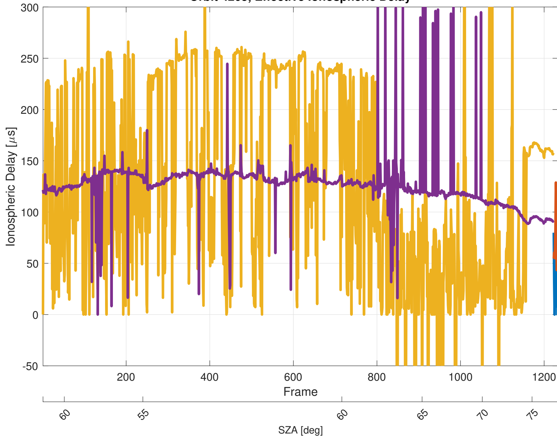
Orbit 4205, Effective Ionospheric Delay
