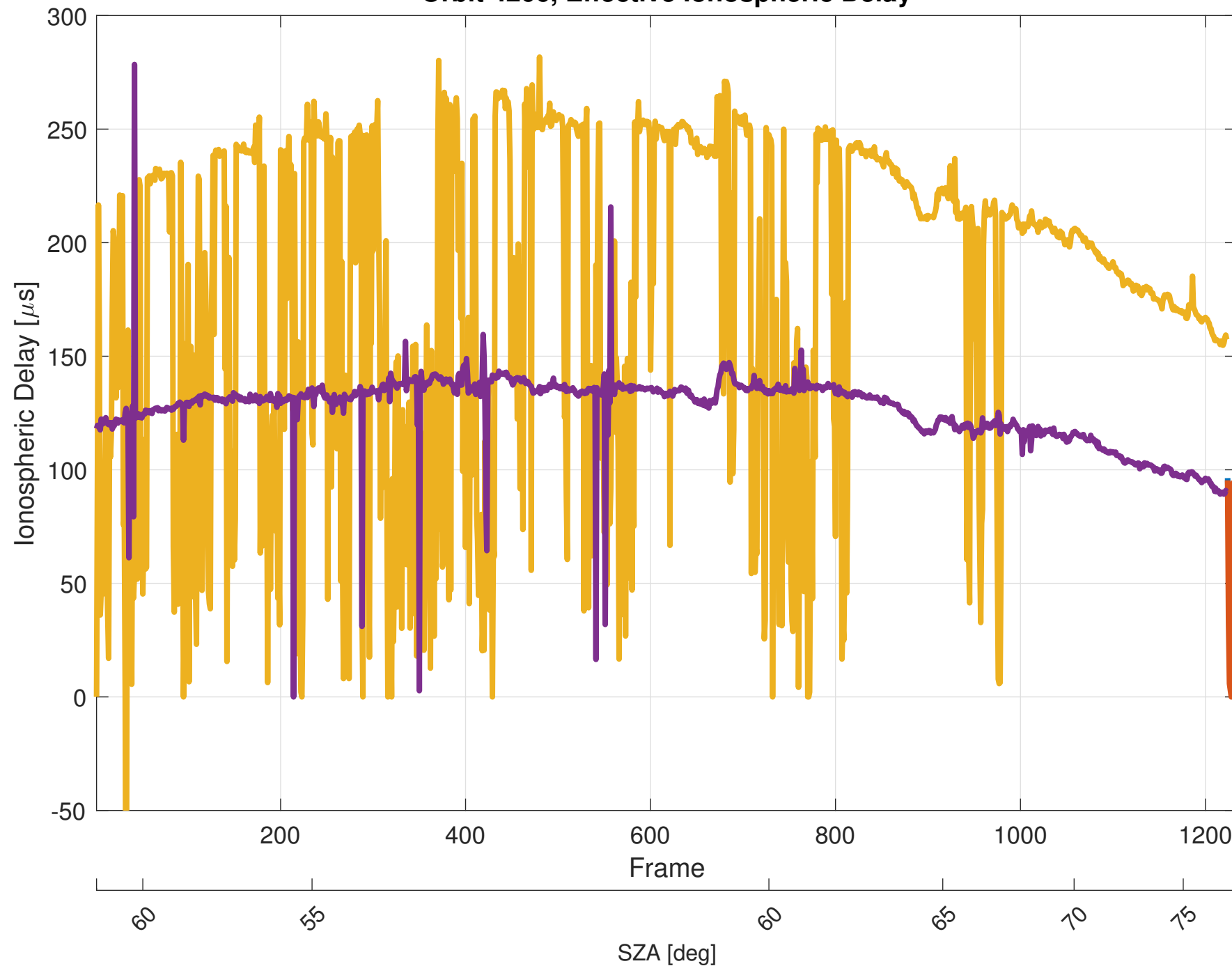
Orbit 4206, Effective Ionospheric Delay
