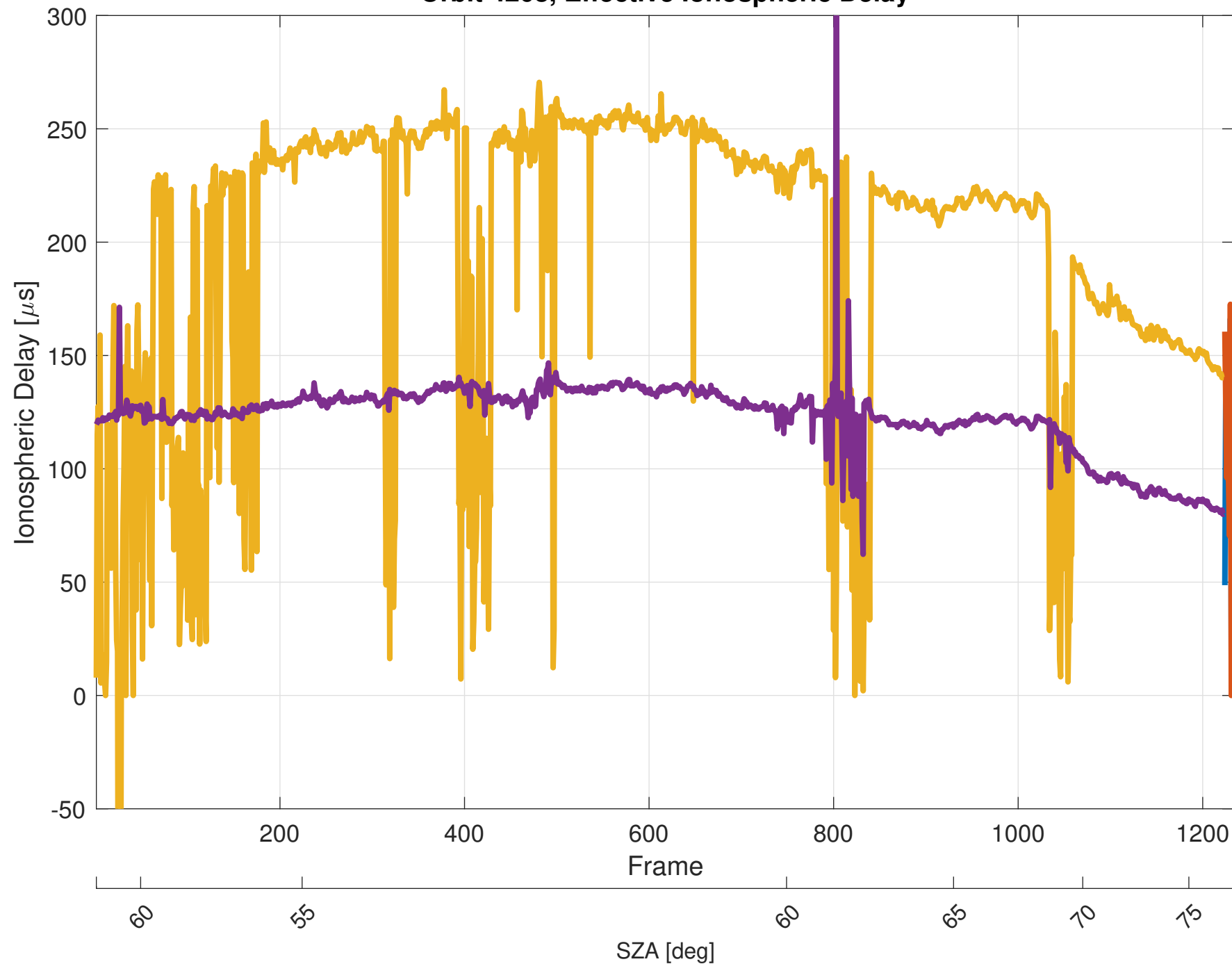
Orbit 4208, Effective Ionospheric Delay
