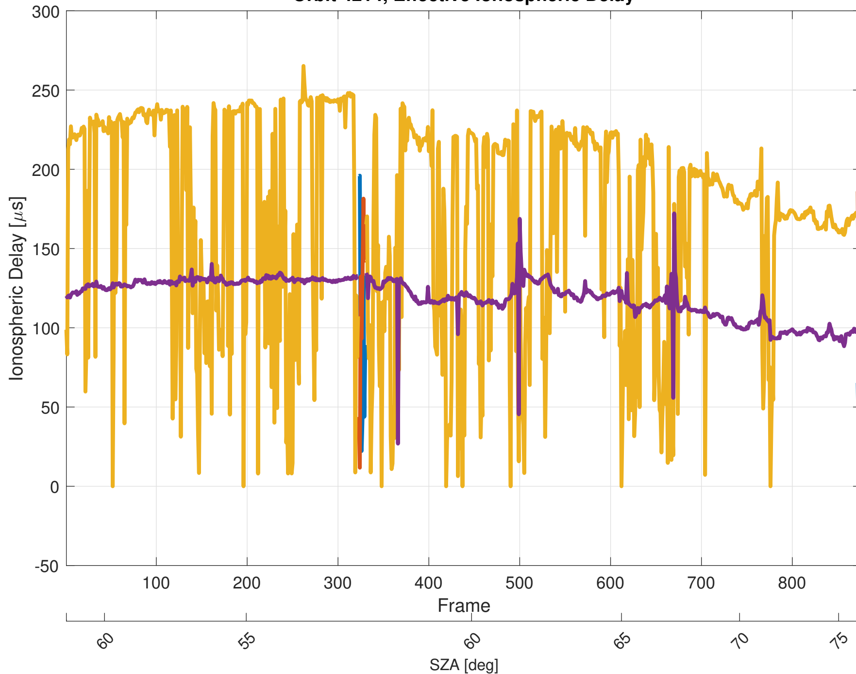
Orbit 4214, Effective Ionospheric Delay
