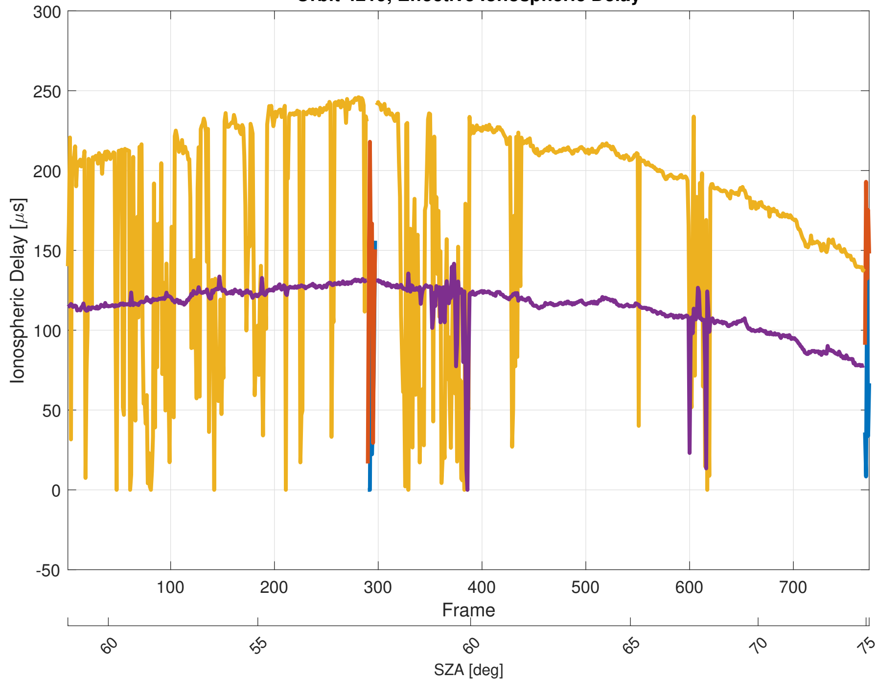
Orbit 4219, Effective Ionospheric Delay
