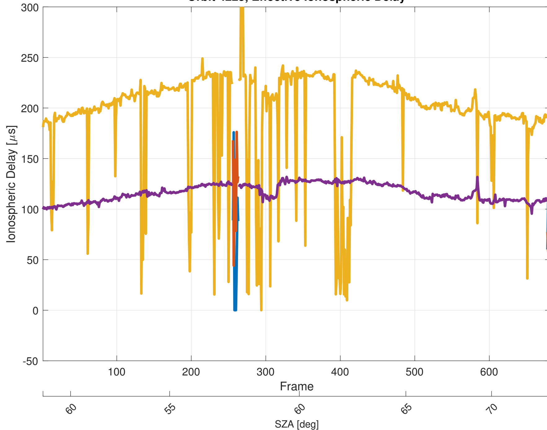
Orbit 4225, Effective Ionospheric Delay
