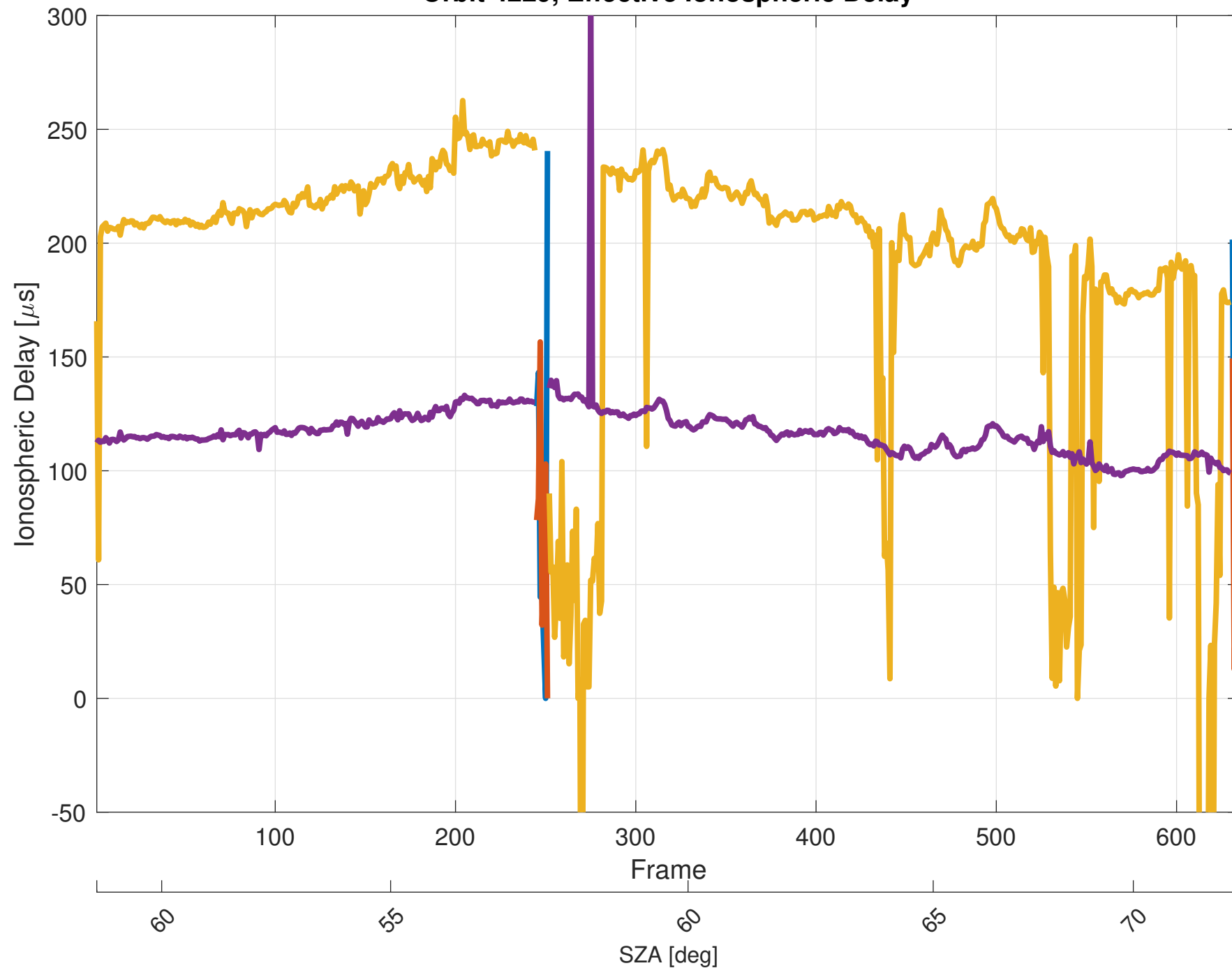
Orbit 4229, Effective Ionospheric Delay
