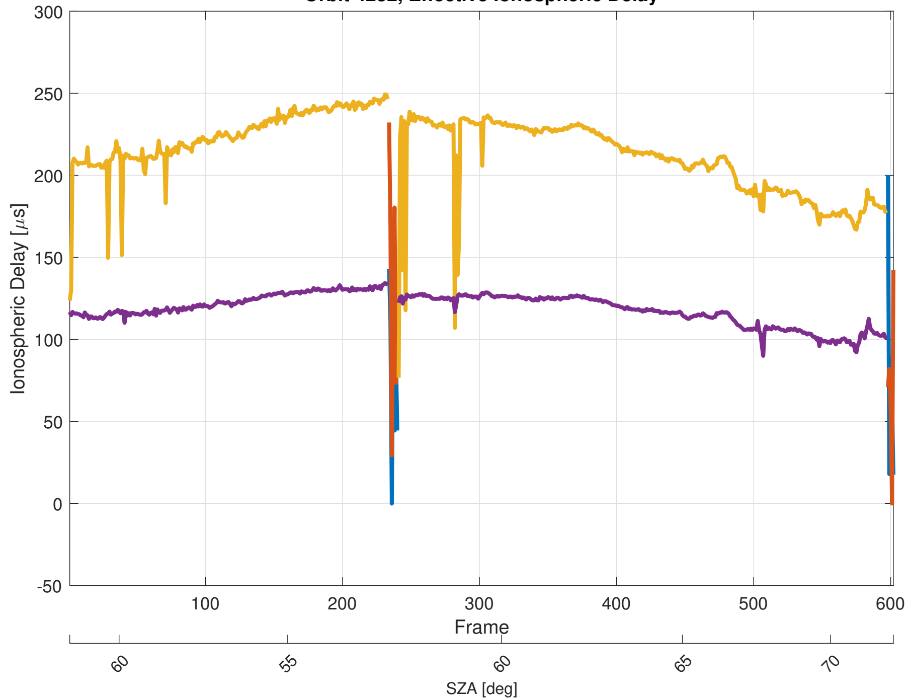
Orbit 4232, Effective Ionospheric Delay
