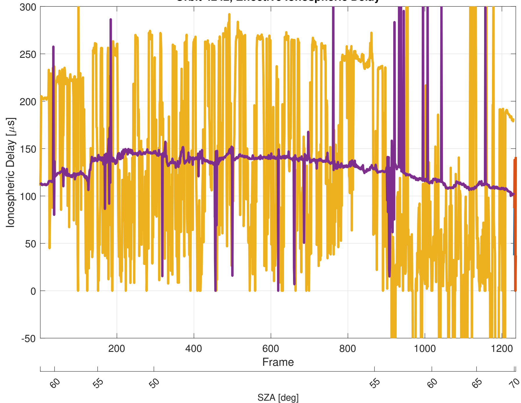
Orbit 4242, Effective Ionospheric Delay
