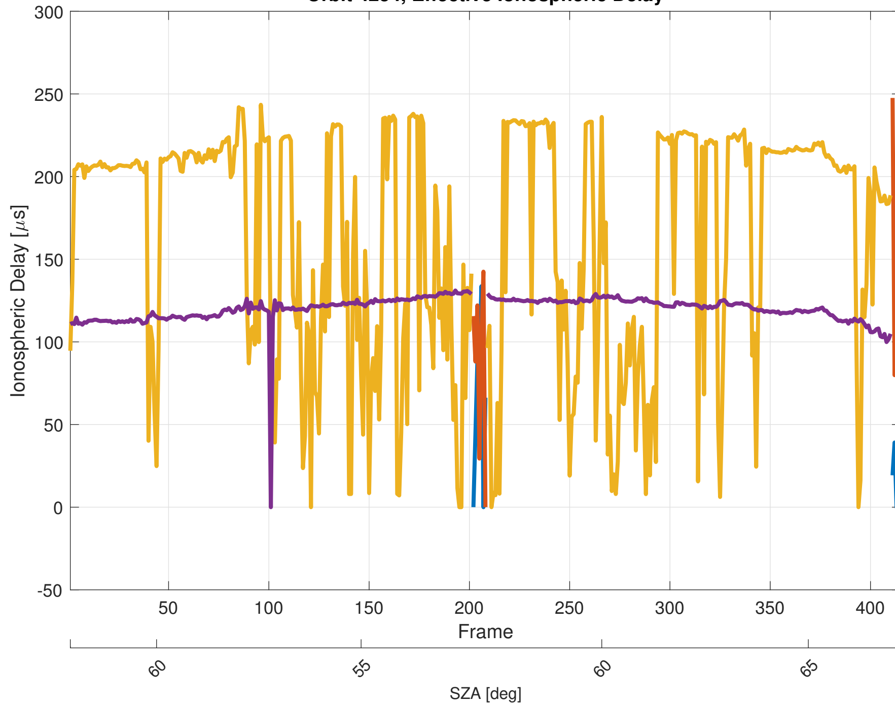
Orbit 4254, Effective Ionospheric Delay
