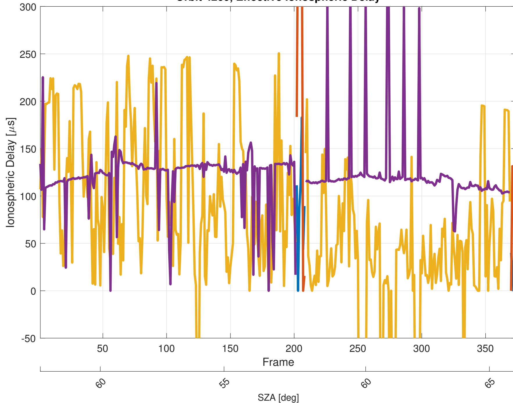
Orbit 4260, Effective Ionospheric Delay
