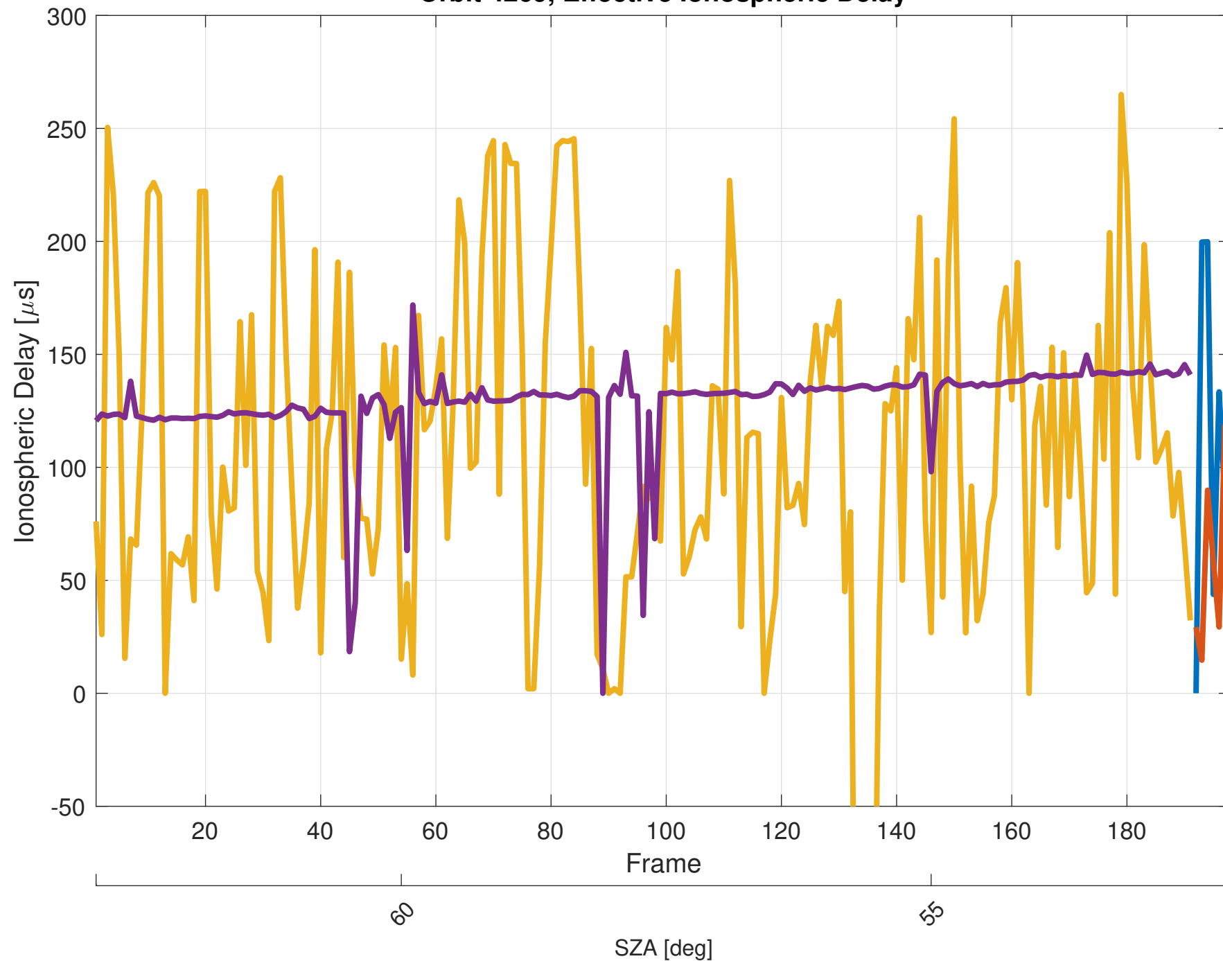
Orbit 4269, Effective Ionospheric Delay
