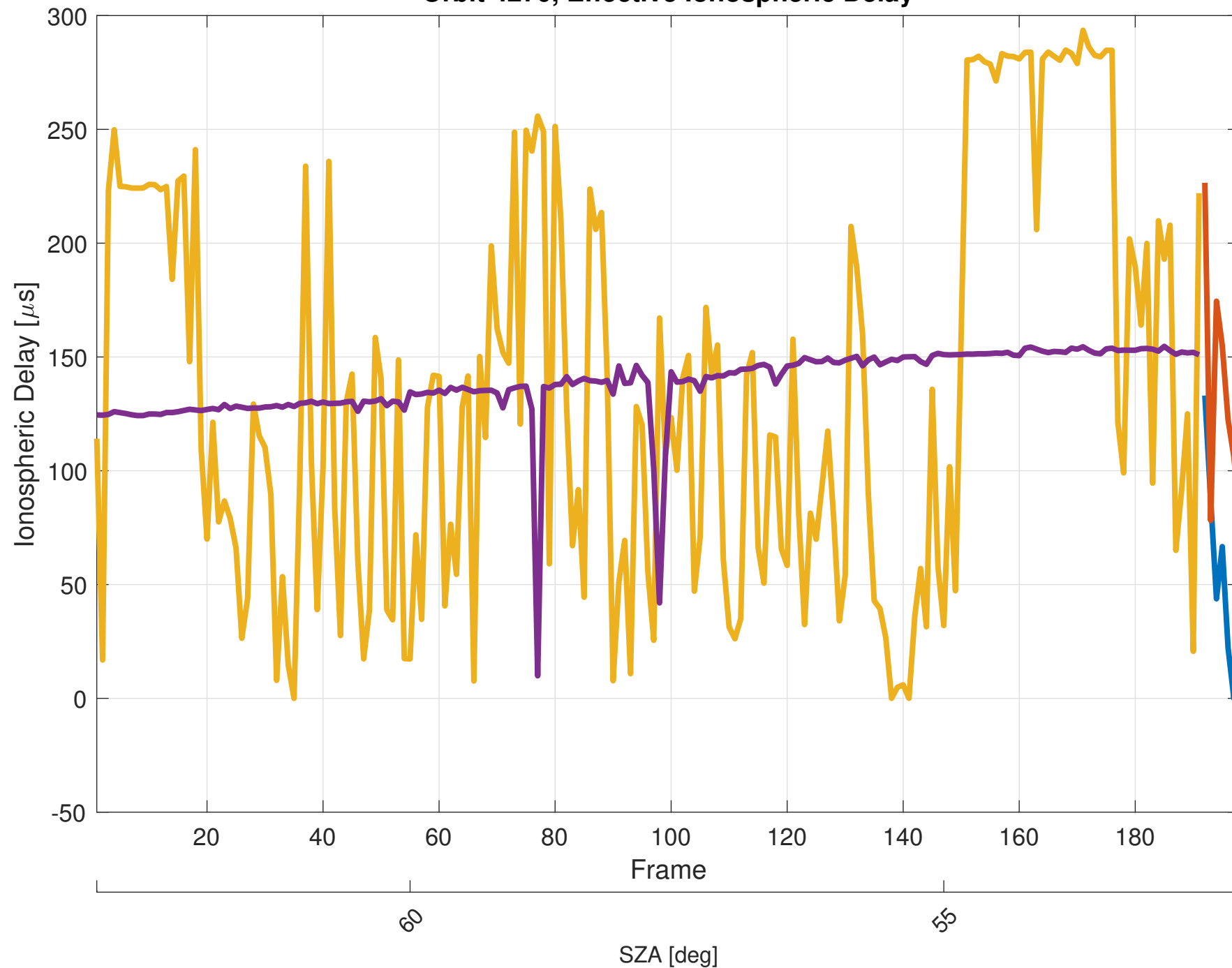
Orbit 4270, Effective Ionospheric Delay
