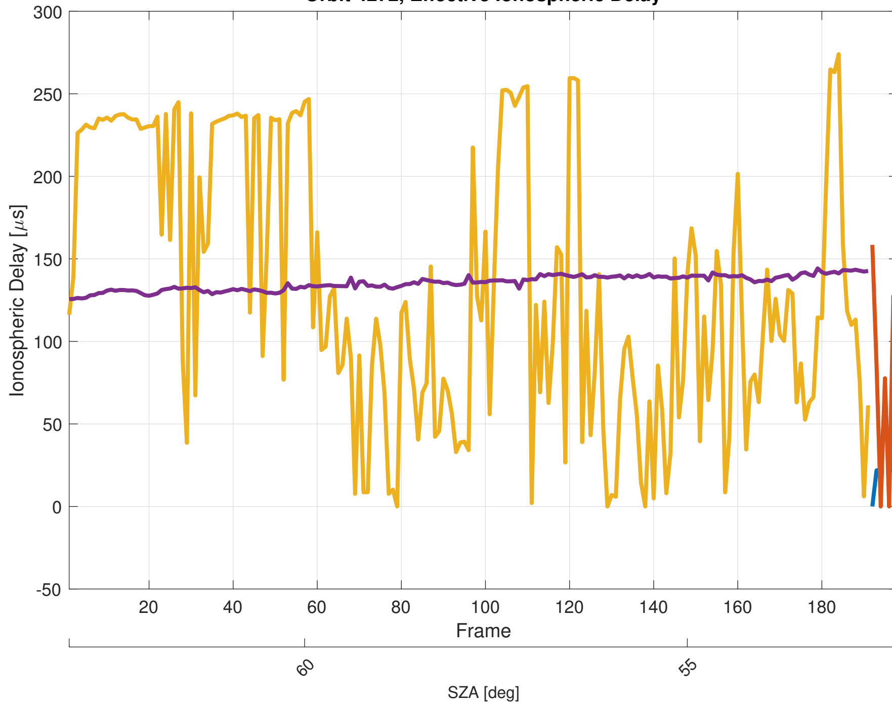
Orbit 4272, Effective Ionospheric Delay
