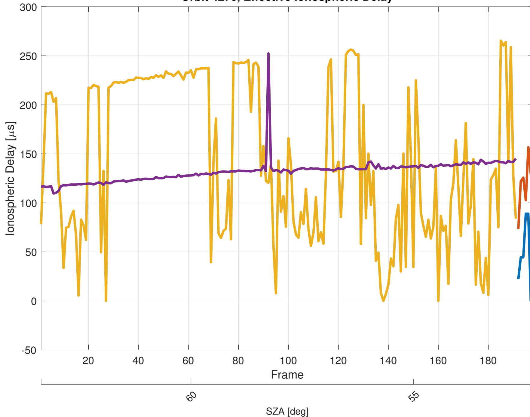
Orbit 4276, Effective Ionospheric Delay
