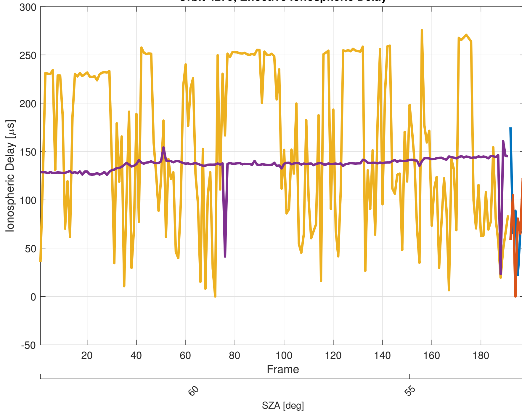
Orbit 4279, Effective Ionospheric Delay
