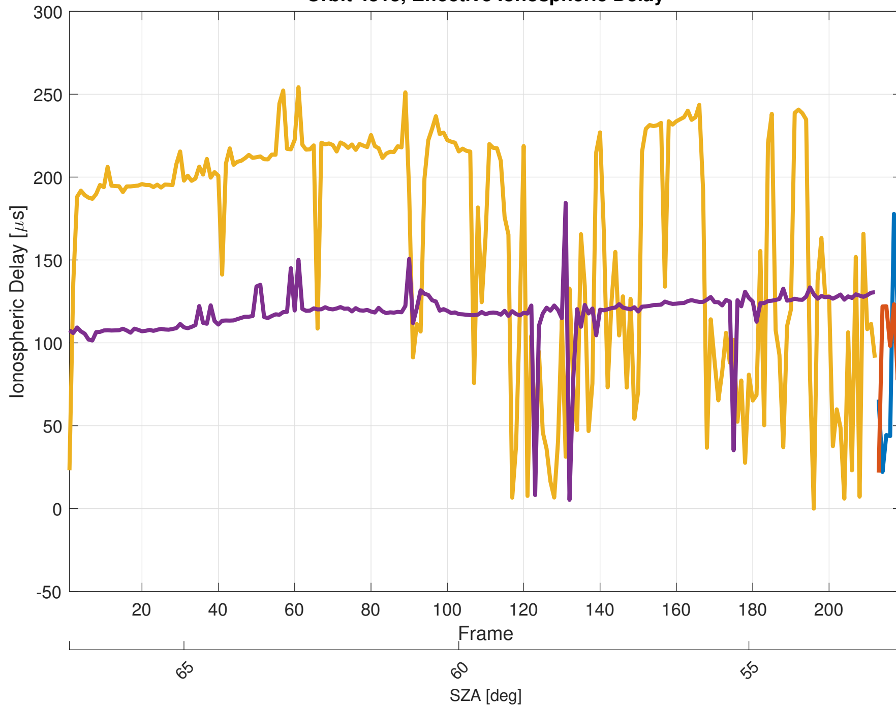
Orbit 4313, Effective Ionospheric Delay
