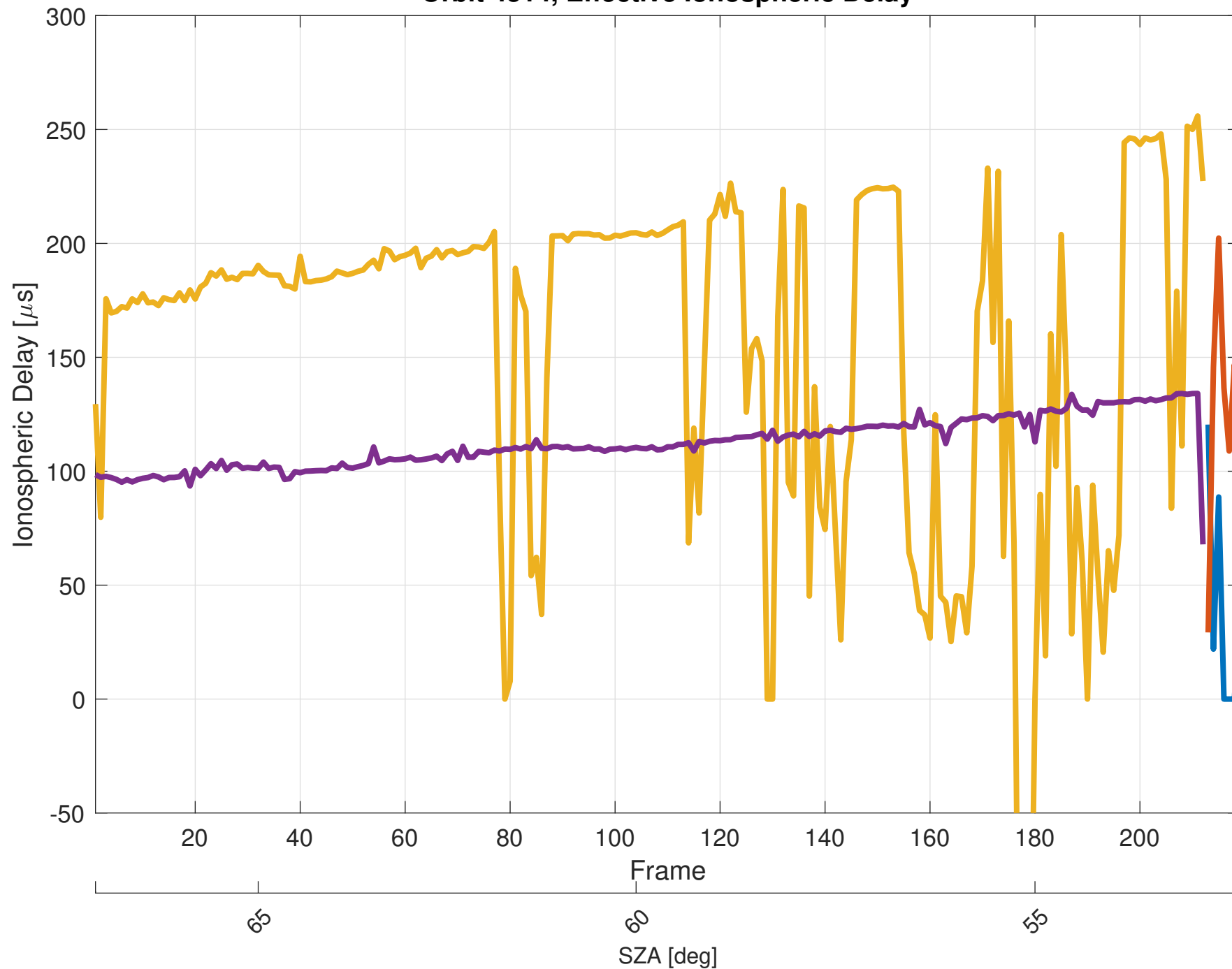
Orbit 4314, Effective Ionospheric Delay
