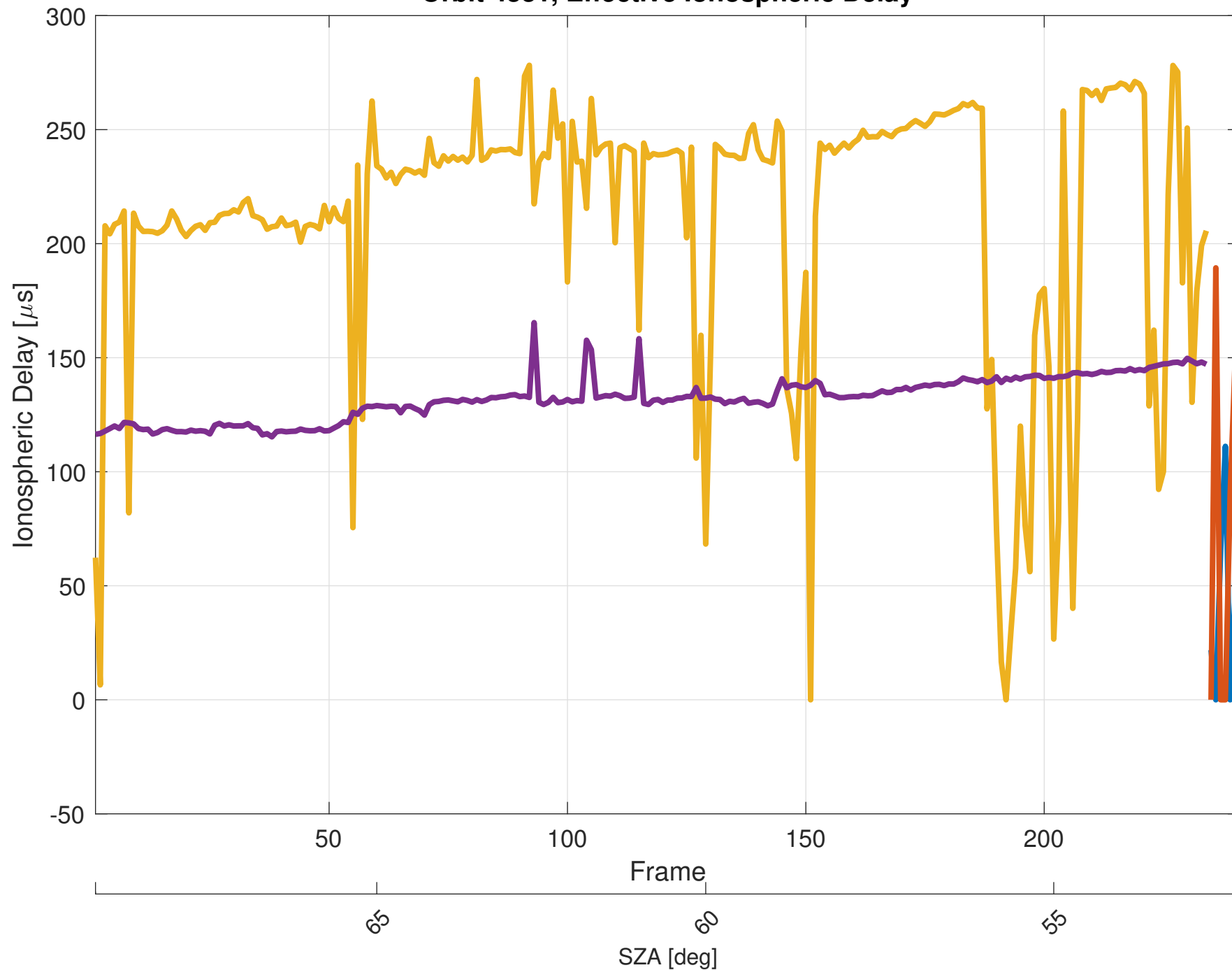
Orbit 4331, Effective Ionospheric Delay
