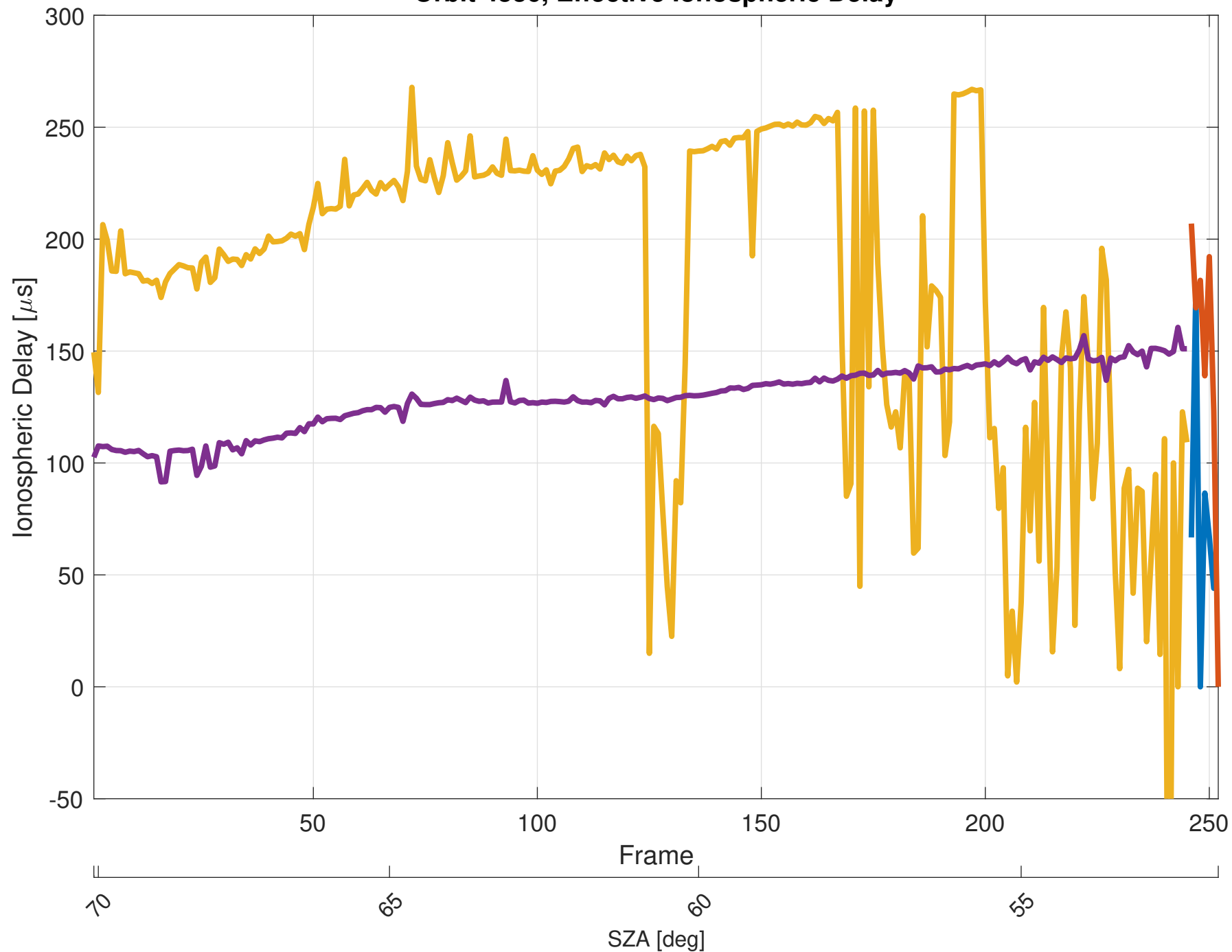
Orbit 4336, Effective Ionospheric Delay
