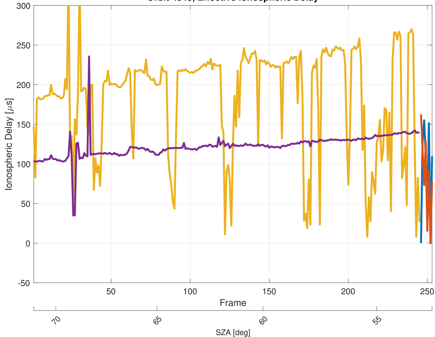
Orbit 4343, Effective Ionospheric Delay
