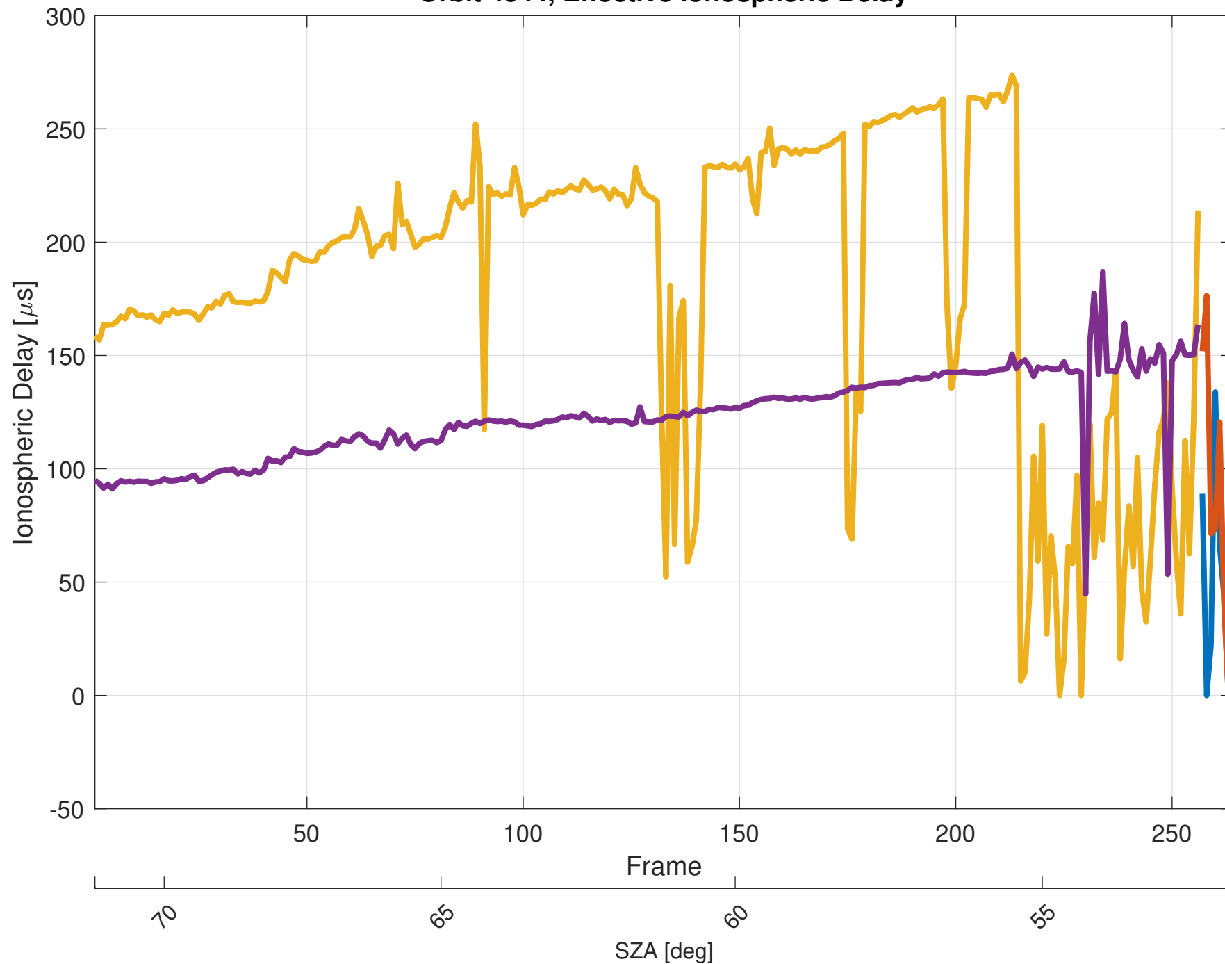
Orbit 4344, Effective Ionospheric Delay
