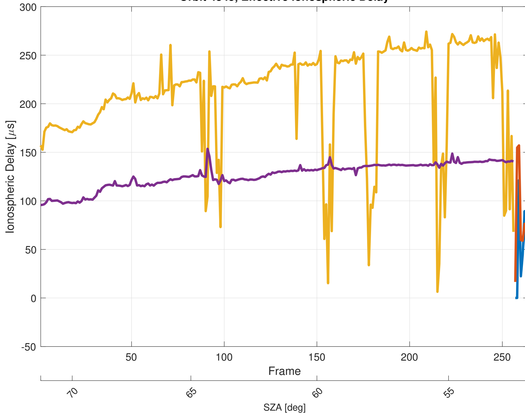
Orbit 4345, Effective Ionospheric Delay
