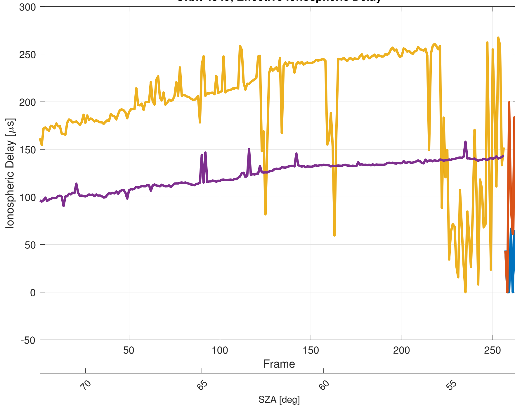
Orbit 4349, Effective Ionospheric Delay
