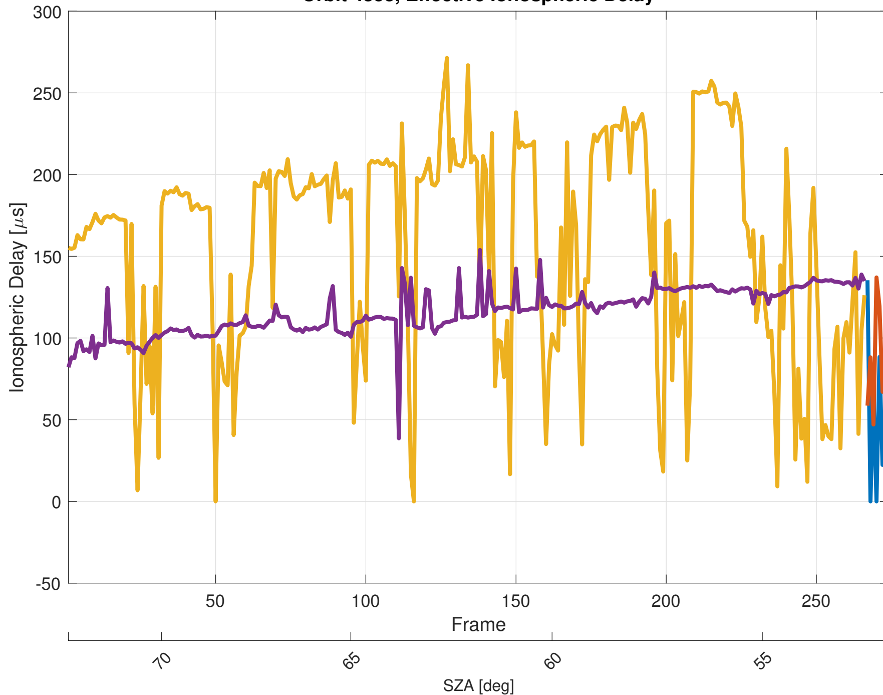
Orbit 4353, Effective Ionospheric Delay
