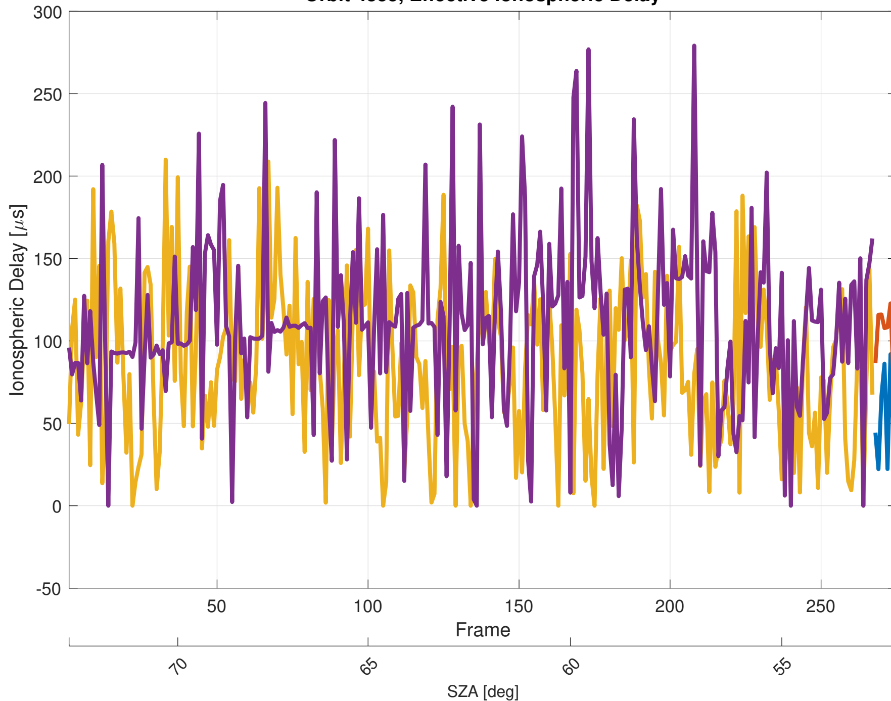
Orbit 4355, Effective Ionospheric Delay
