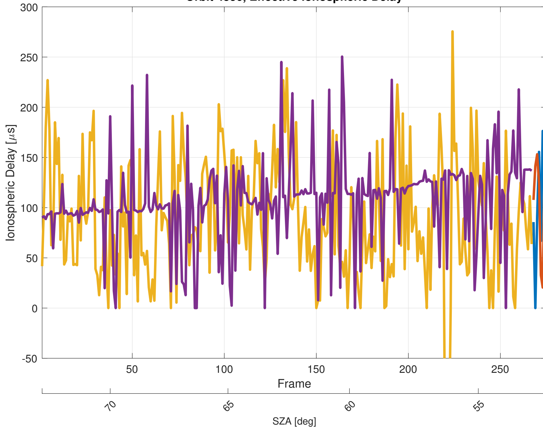
Orbit 4356, Effective Ionospheric Delay
