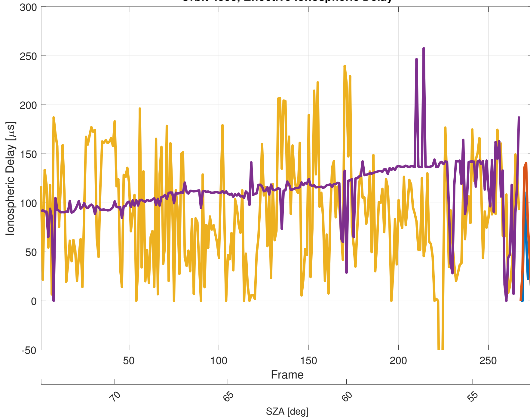
Orbit 4358, Effective Ionospheric Delay
