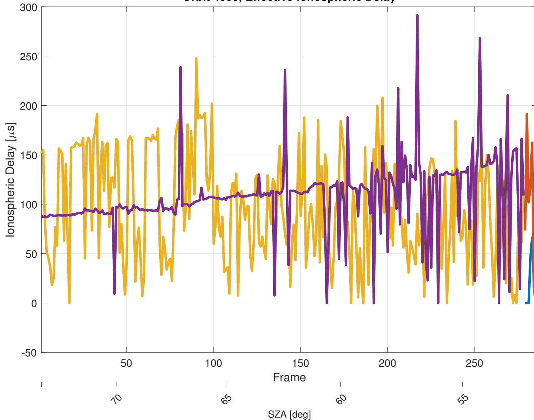
Orbit 4359, Effective Ionospheric Delay
