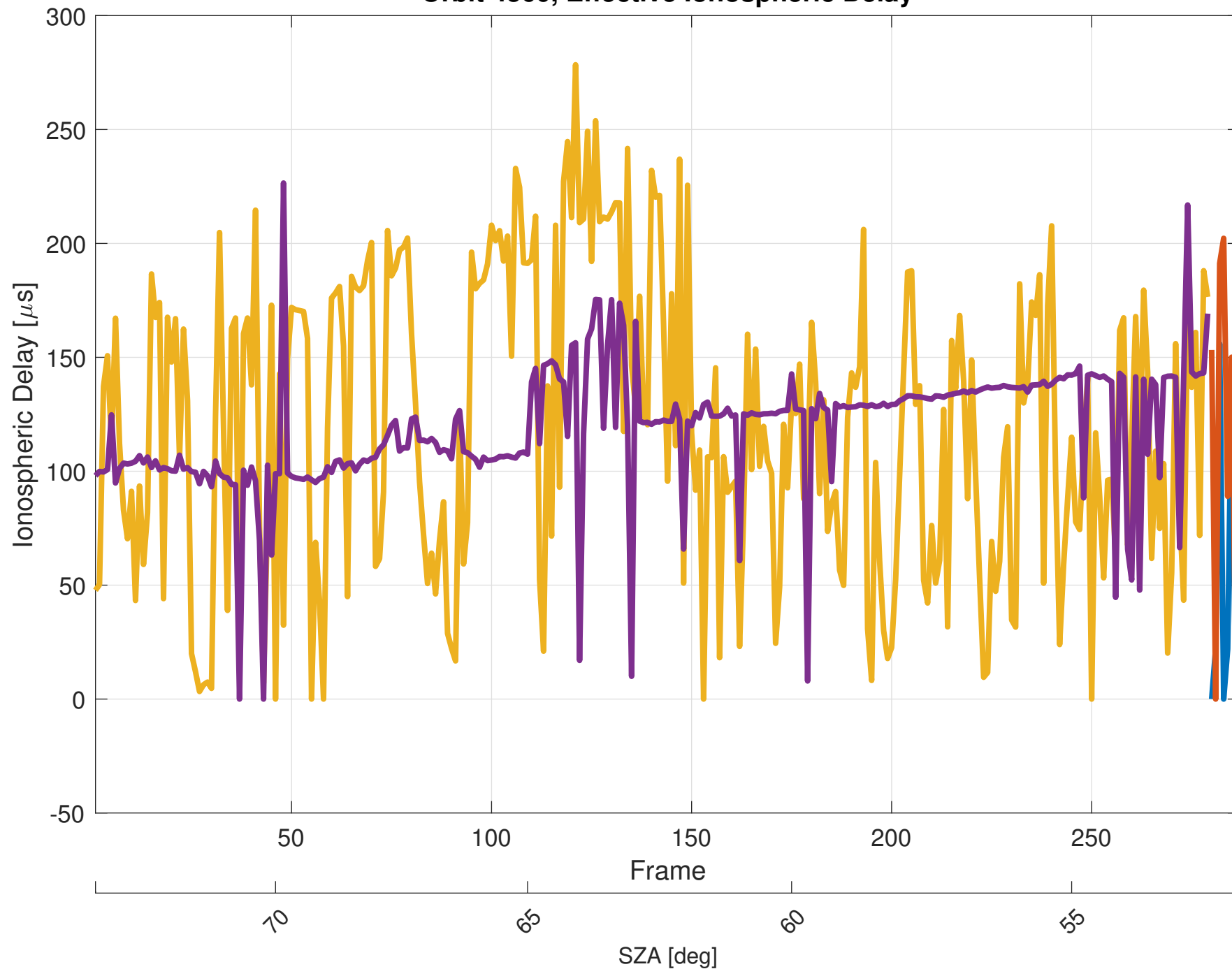
Orbit 4360, Effective Ionospheric Delay
