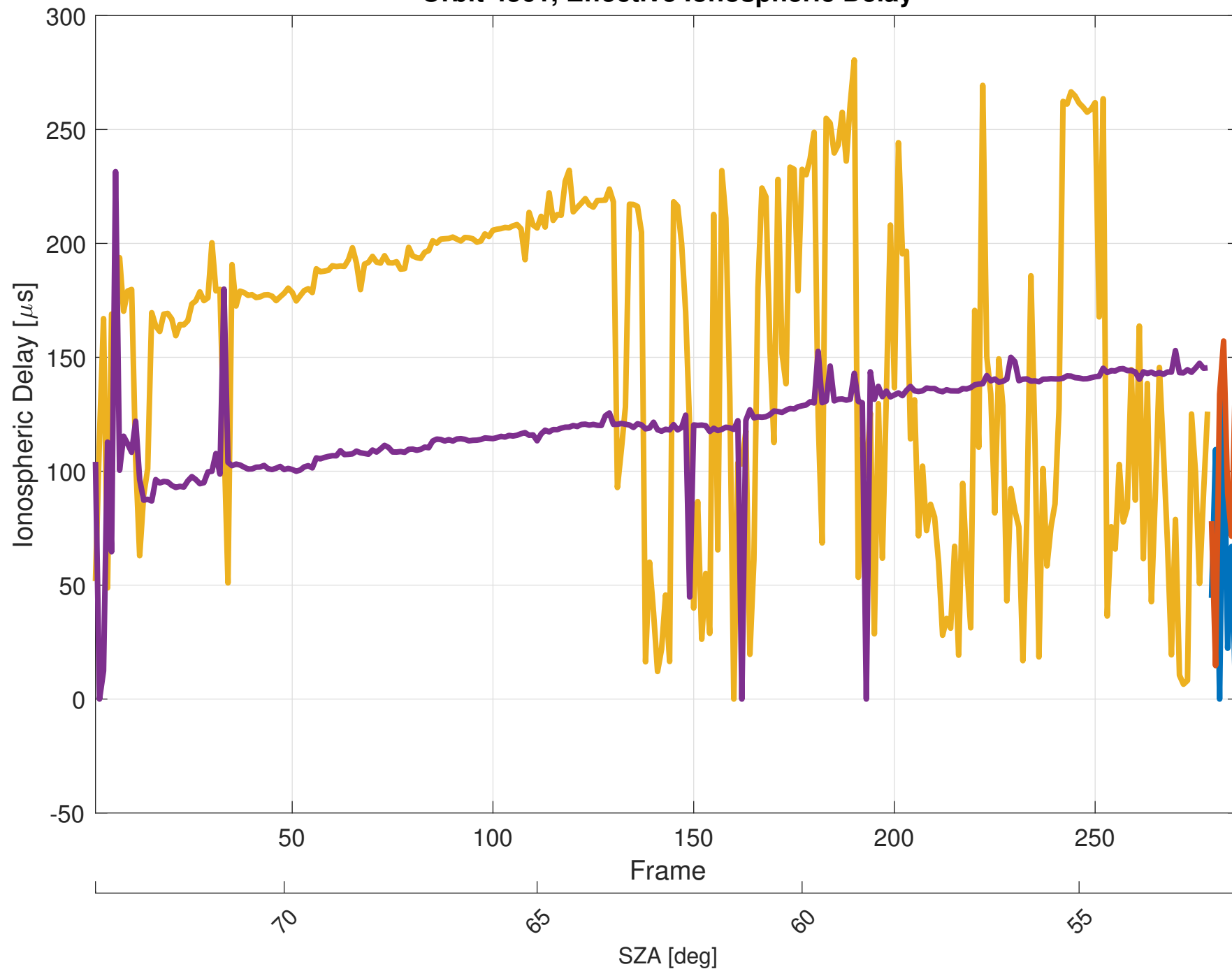
Orbit 4361, Effective Ionospheric Delay
