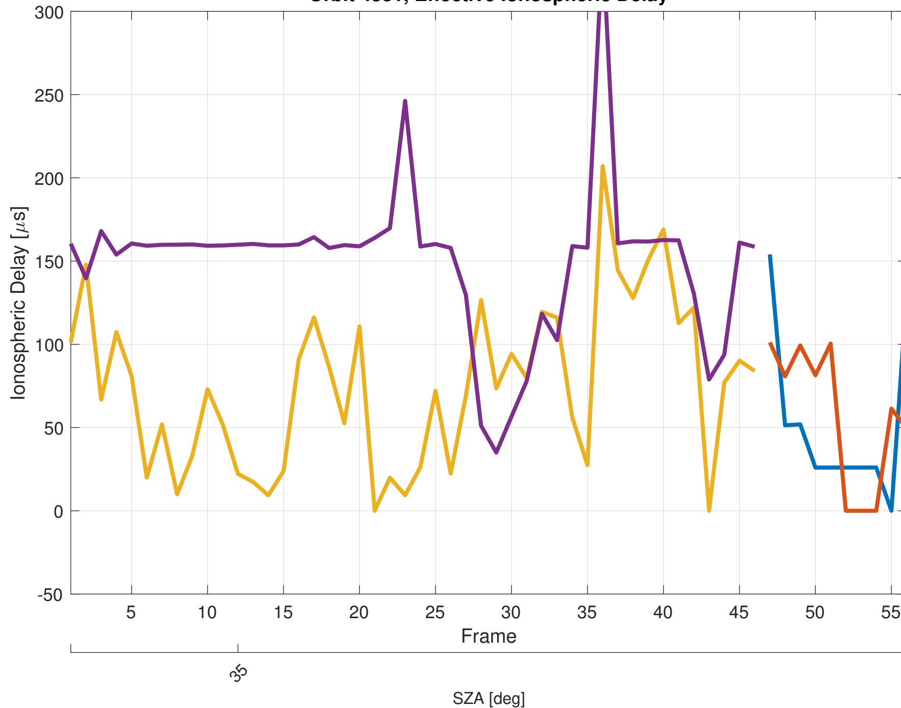
Orbit 4381, Effective Ionospheric Delay
