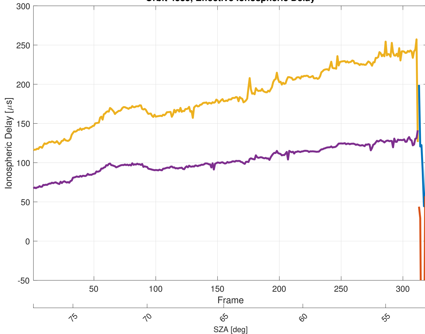
Orbit 4385, Effective Ionospheric Delay
