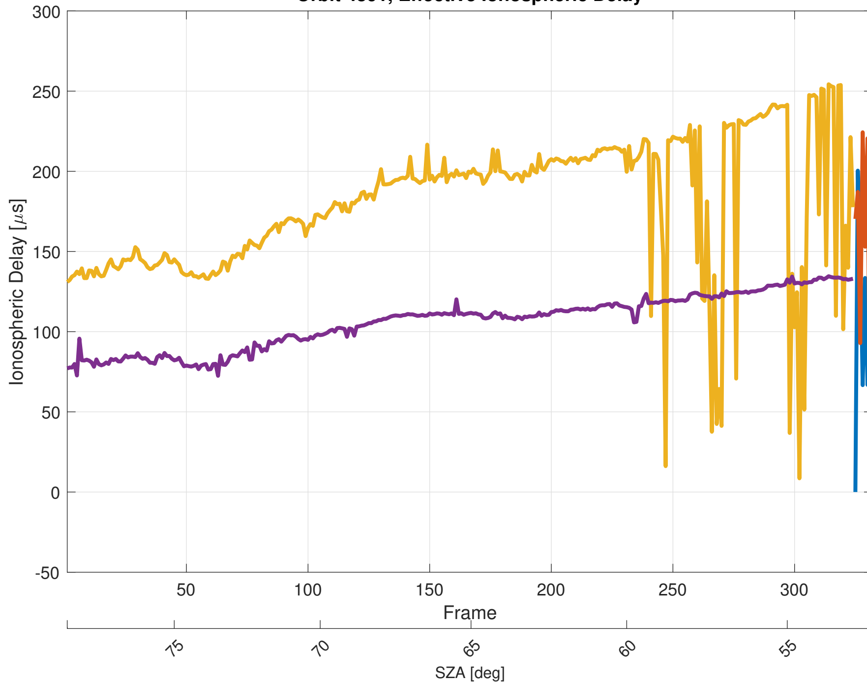
Orbit 4391, Effective Ionospheric Delay
