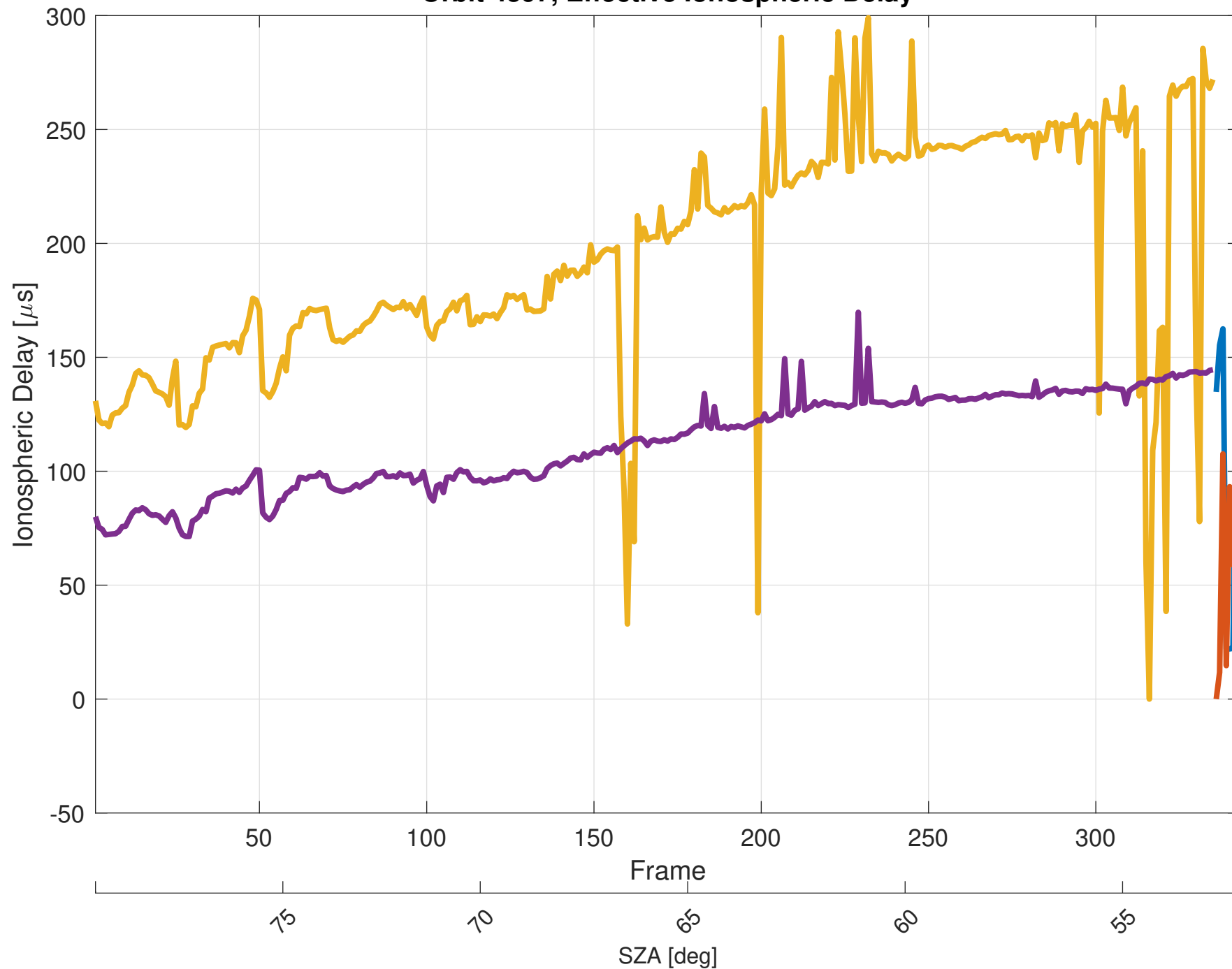
Orbit 4397, Effective Ionospheric Delay
