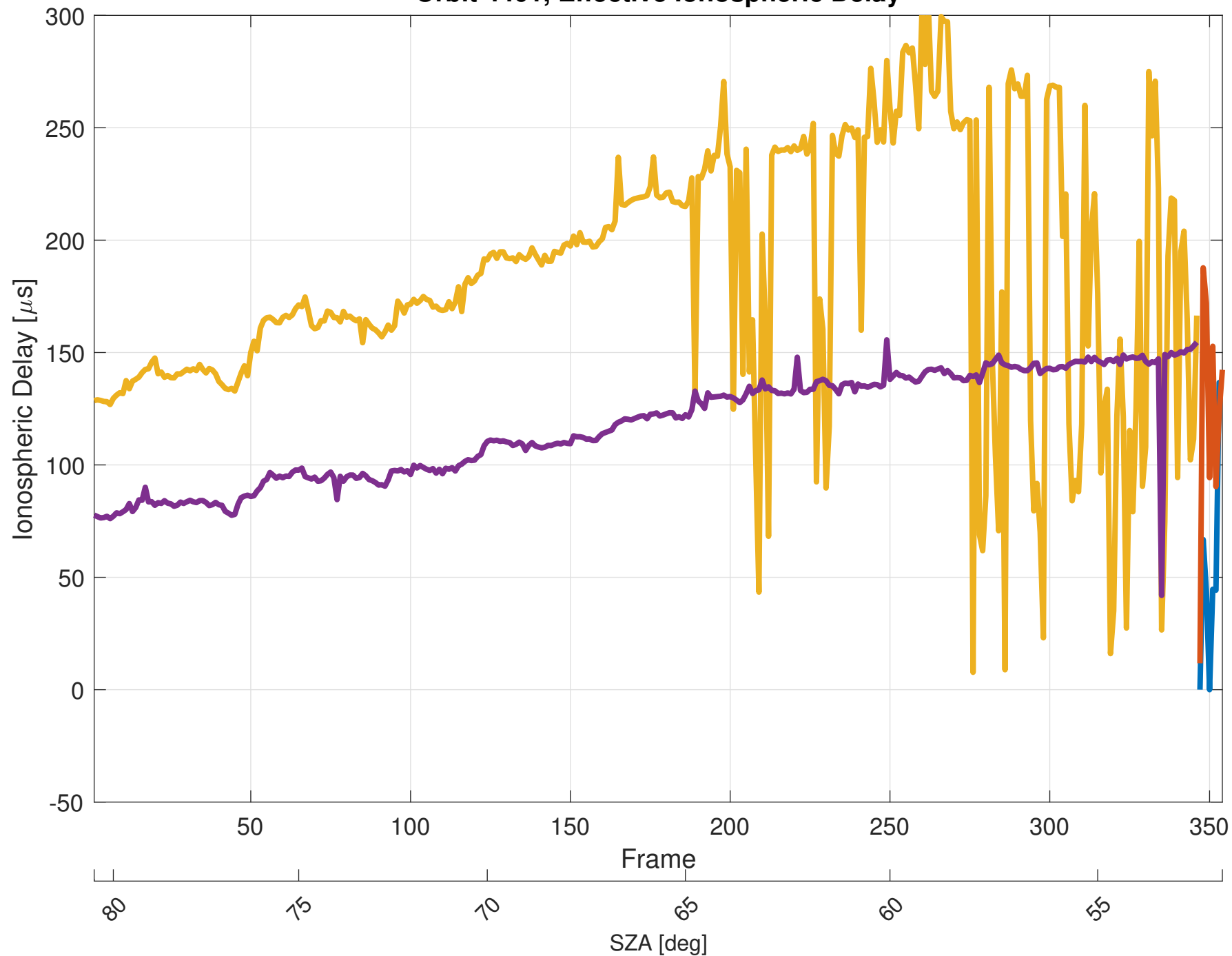
Orbit 4401, Effective Ionospheric Delay
