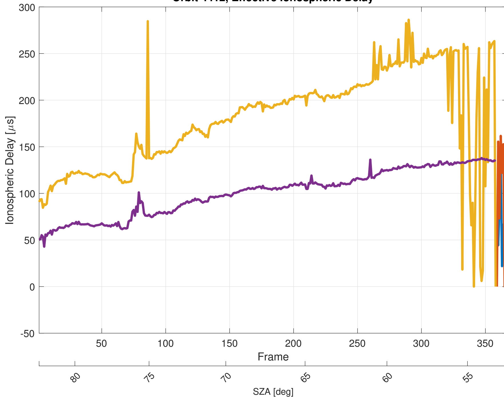
Orbit 4412, Effective Ionospheric Delay
