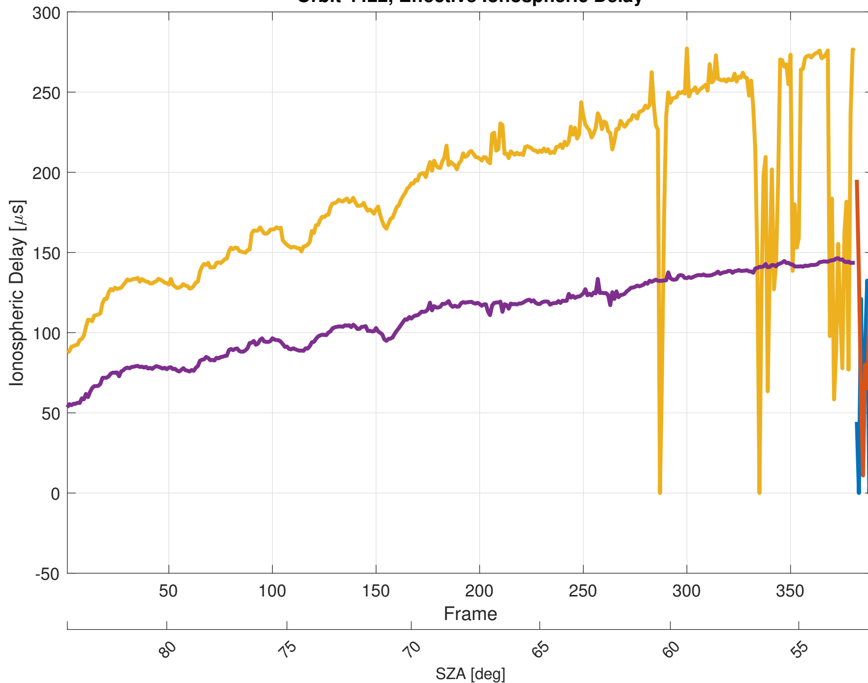
Orbit 4422, Effective Ionospheric Delay
