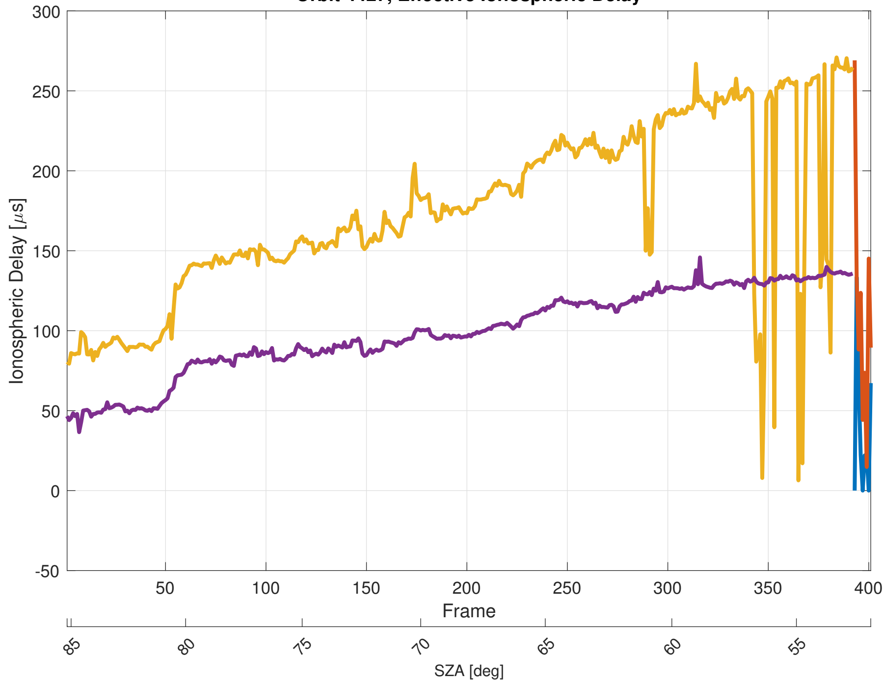
Orbit 4427, Effective Ionospheric Delay
