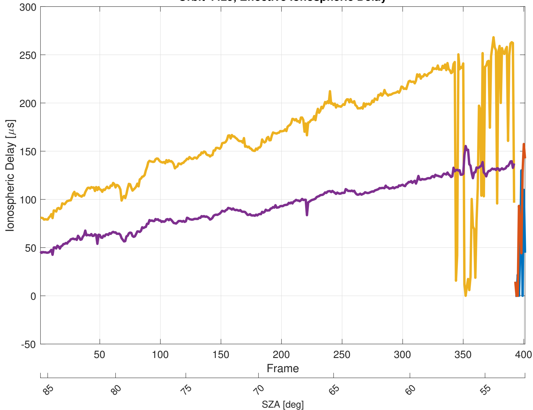
Orbit 4429, Effective Ionospheric Delay
